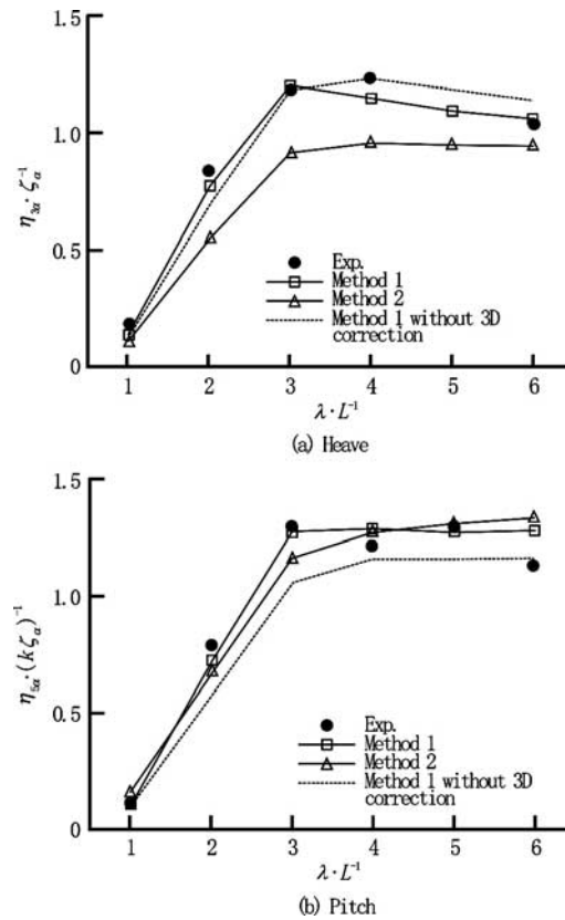
Fig. 4 Heave and pitch amplitudes by different methods
