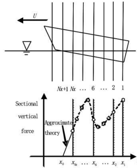
Fig. 2 Numerical strategy of the 2D+t calculations
