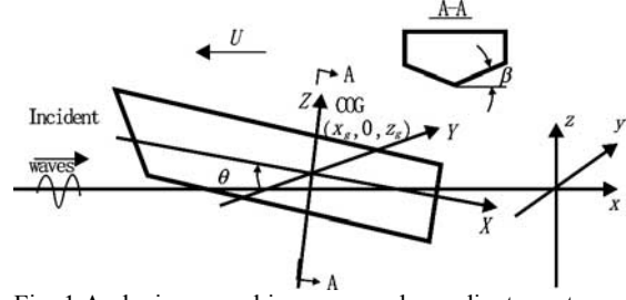
Fig. 1 A planing vessel in waves and coordinate systems
