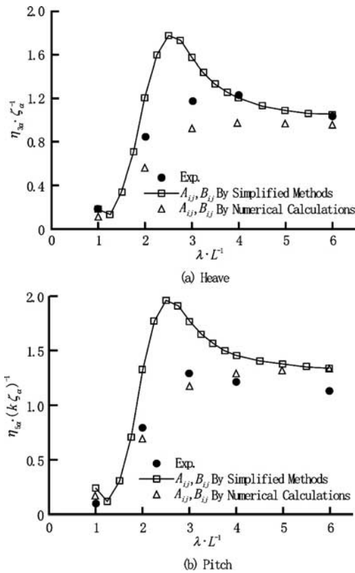
Fig. 3 Heave and pitch amplitudes by simplified methods
