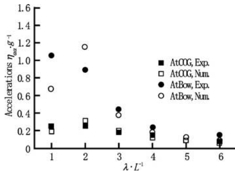
Fig. 6 Accelerations at the COG and at the bow
